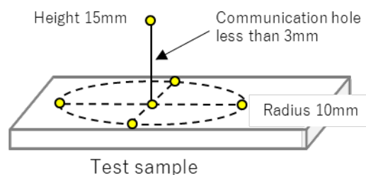
Interoperability Test
