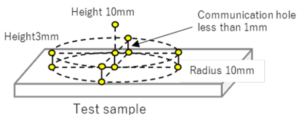
Basic Performance Test
