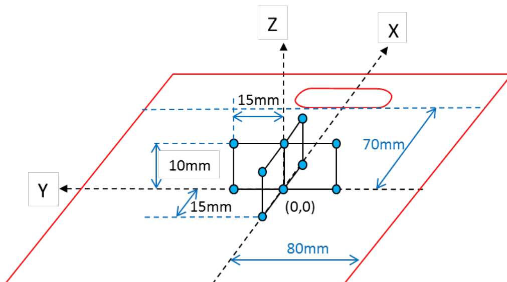
Figure 6-16 Out-of-range communication measurement points
