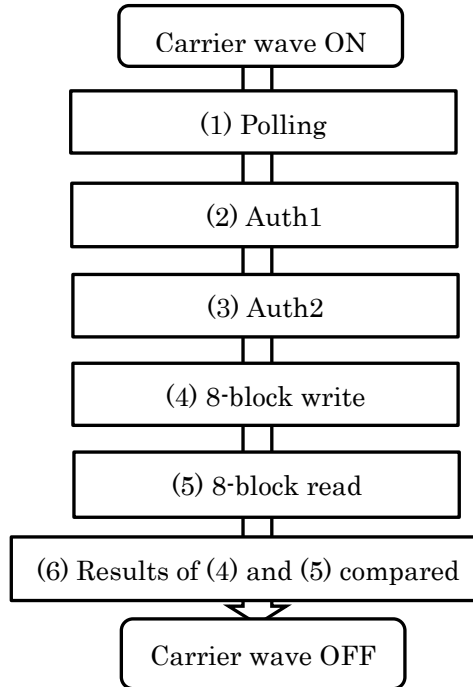
Figure 6-20 Sequence Software
