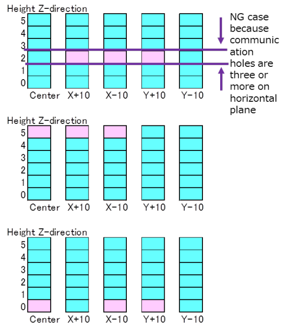
Figure 6-14 Example2: Pass/Fail Criteria for Center, Offset
